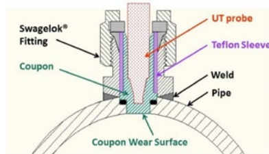
Schematic showing coupon installed in a pipe
